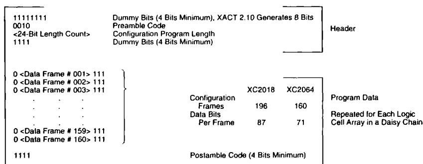
Figure 12. XC2064 Internal Configuration Data Arrangement
