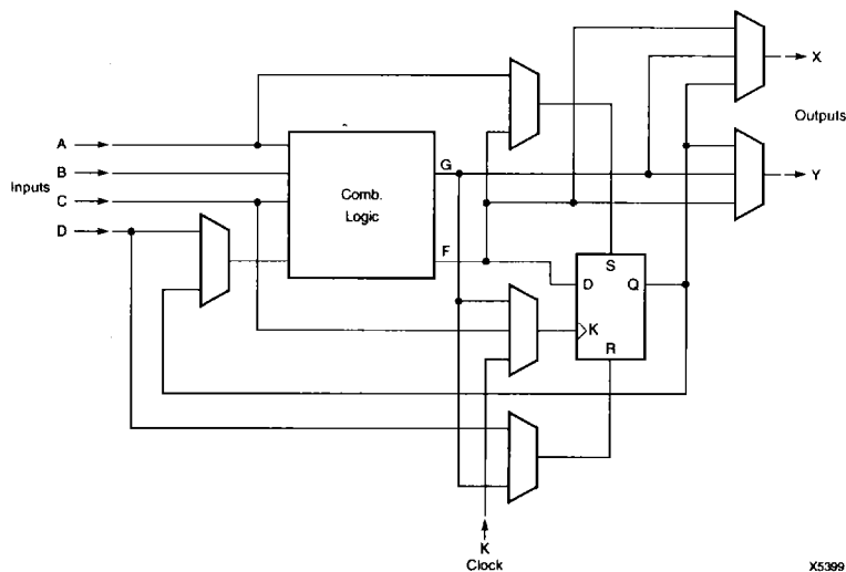
Figure 4. Configurable Logic Block
