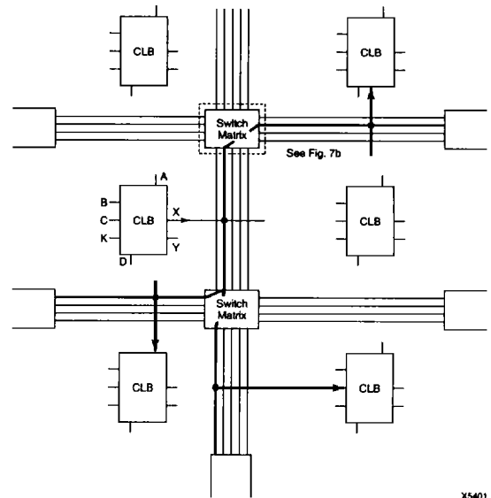
Figure 7a. General-Purpose Interconnect
