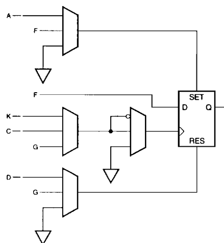
Figure 6. CLB Storage Element
