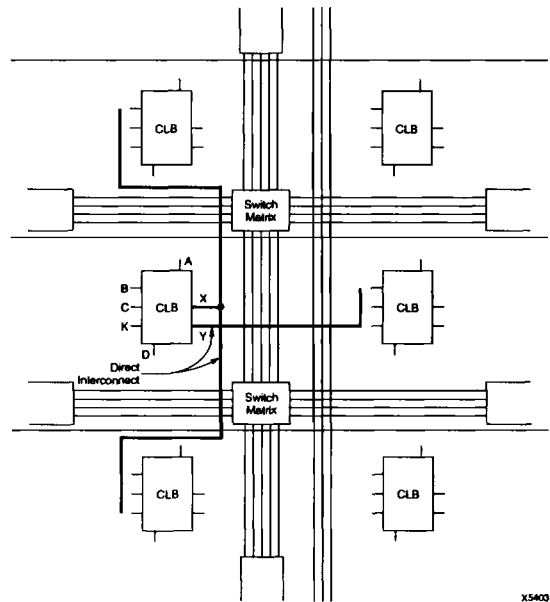
Figure 9. Direct Interconnect
